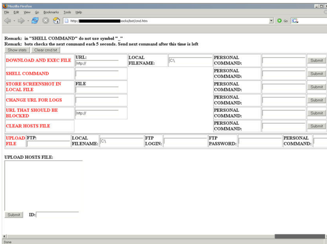
Figure 9 - Web -based Command and Control - Command Interface
